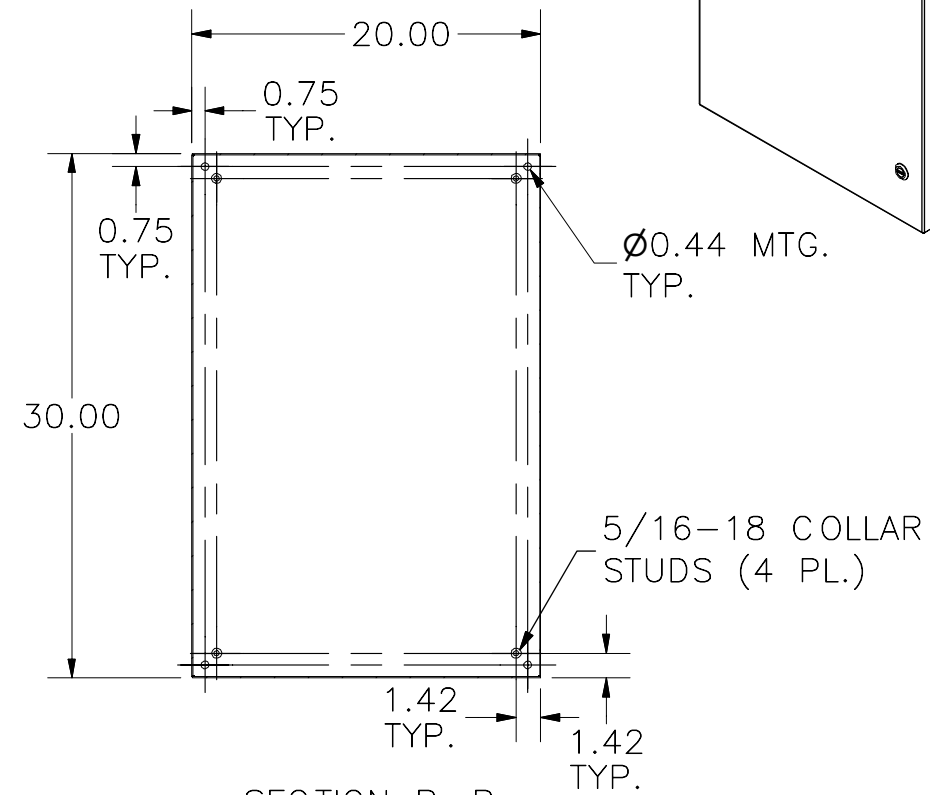
SECTION B-B (INSIDE BACK OF ENCLOSURE)
