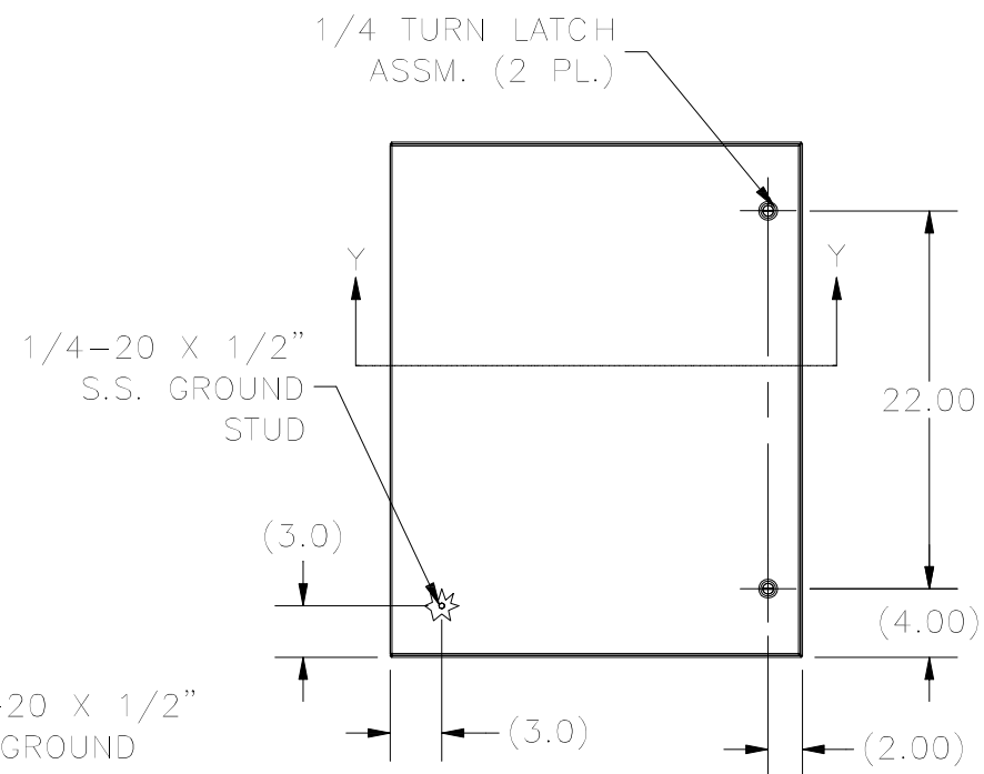
FRONT VIEW
