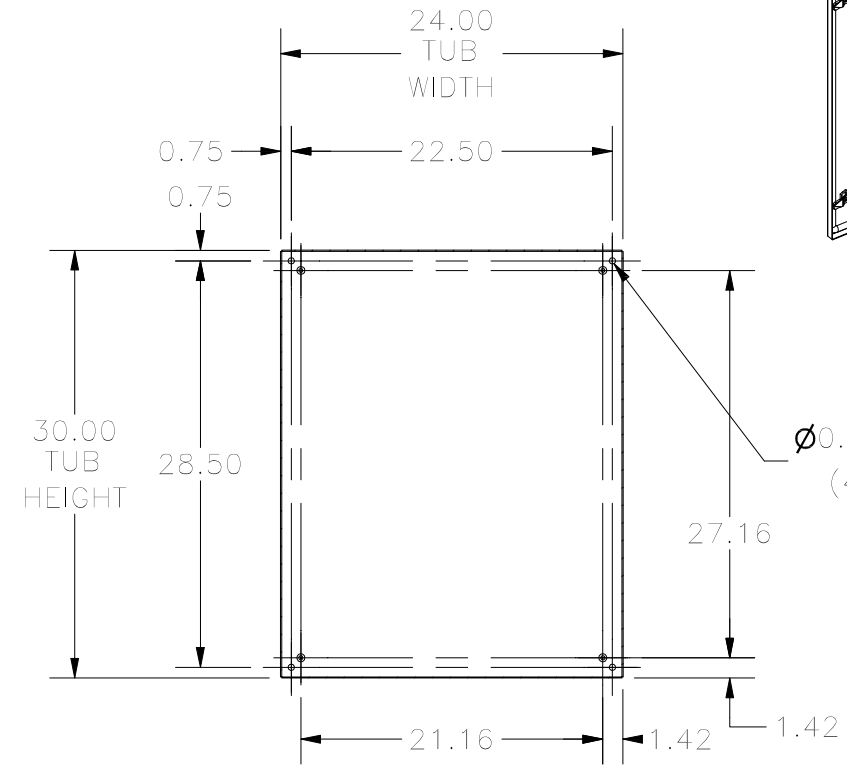
SECTION Y-Y (INSIDE BACK OF ENCLOSURE)
