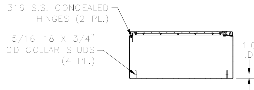
SECTION AA-AA (INSIDE TOP OF ENCLOSURE)
