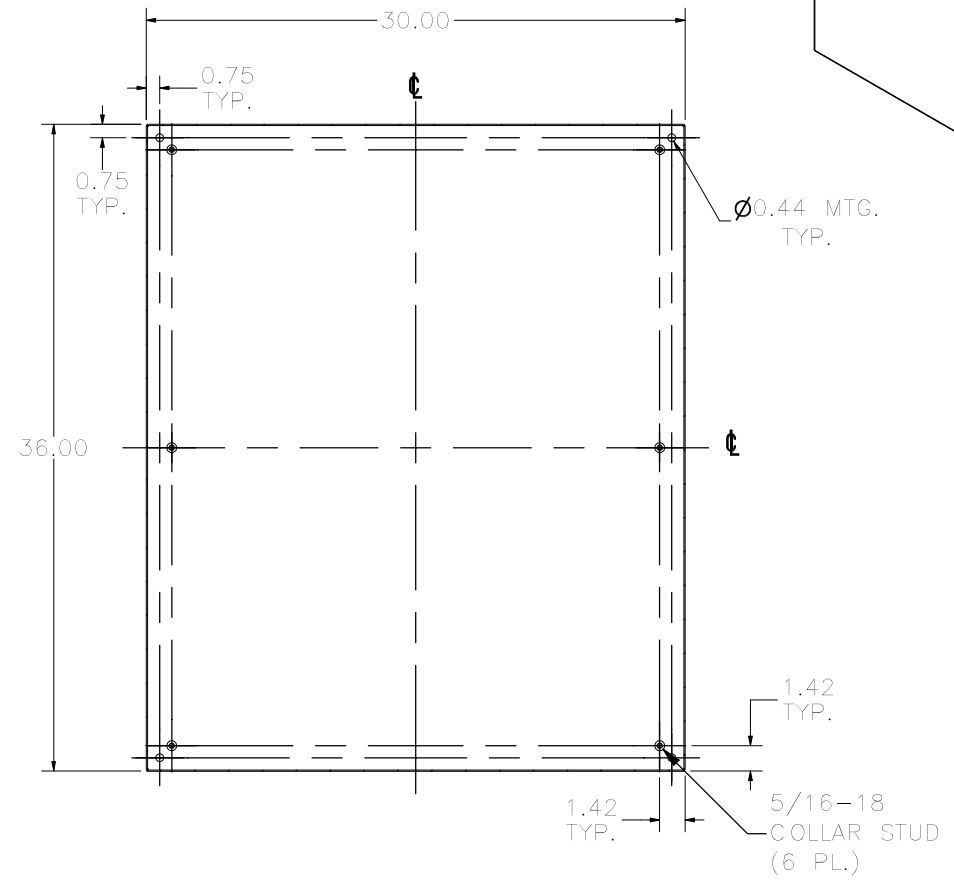
SECTION D-D VIEW (INSIDE BACK OF ENCLOSURE)
