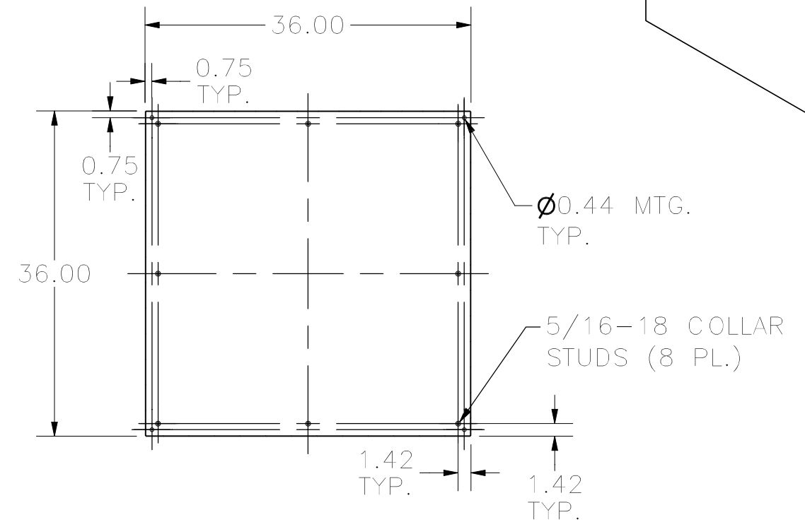
SECTION A-A (INSIDE BACK OF ENCLOSURE)
