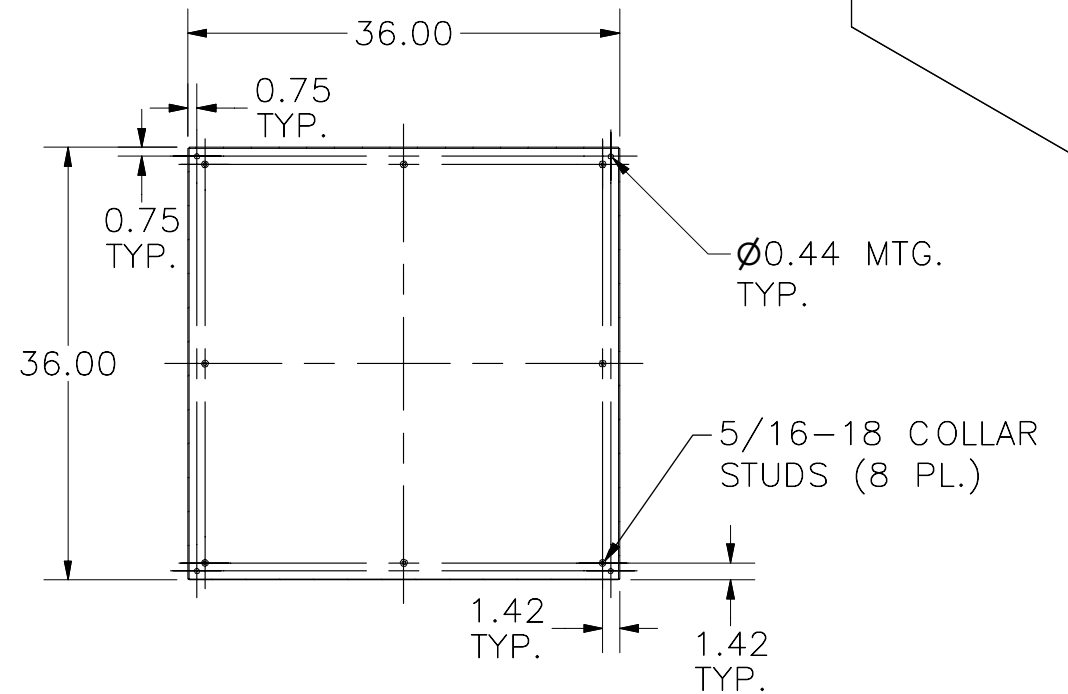
SECTION A-A (INSIDE BACK OF ENCLOSURE)
