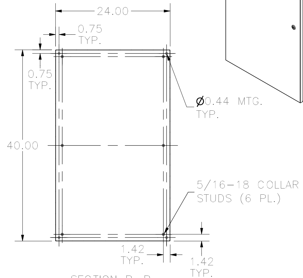
SECTION B-B (INSIDE BACK OF ENCLOSURE)
