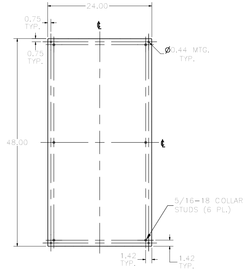
SECTION E-E VIEW (INSIDE BACK OF ENCLOSURE)
