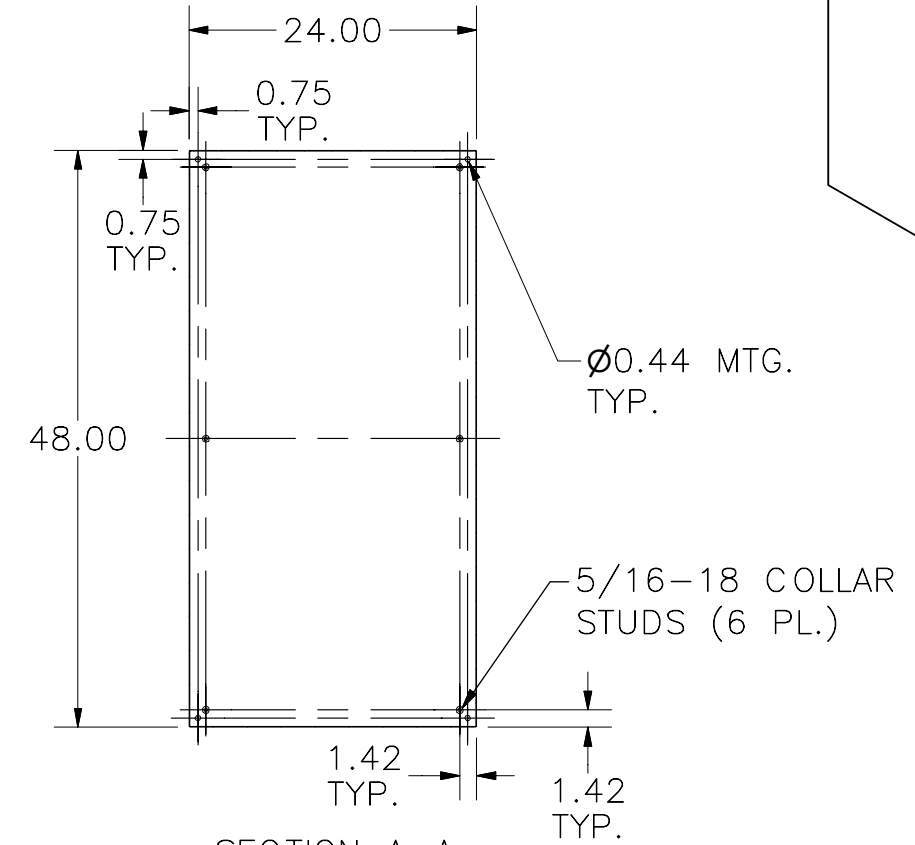
SECTION A-A (INSIDE BACK OF ENCLOSURE)
