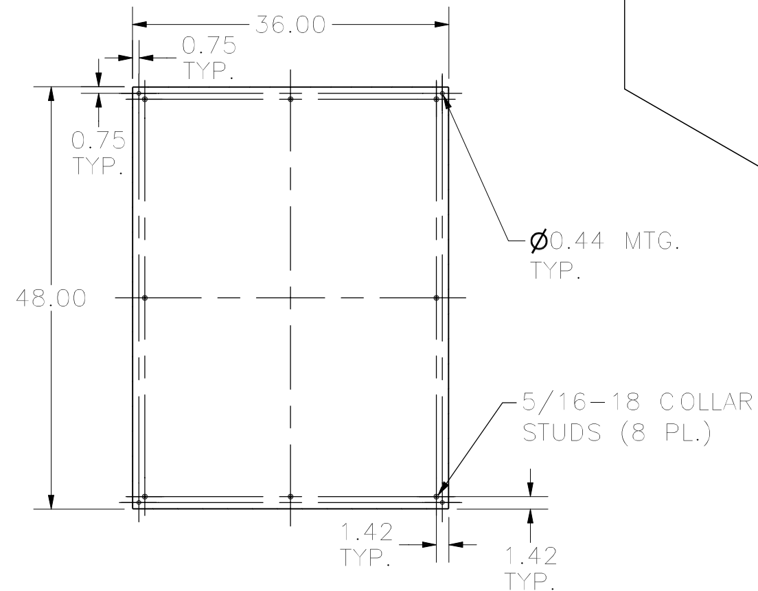
SECTION A-A (INSIDE BACK OF ENCLOSURE)
