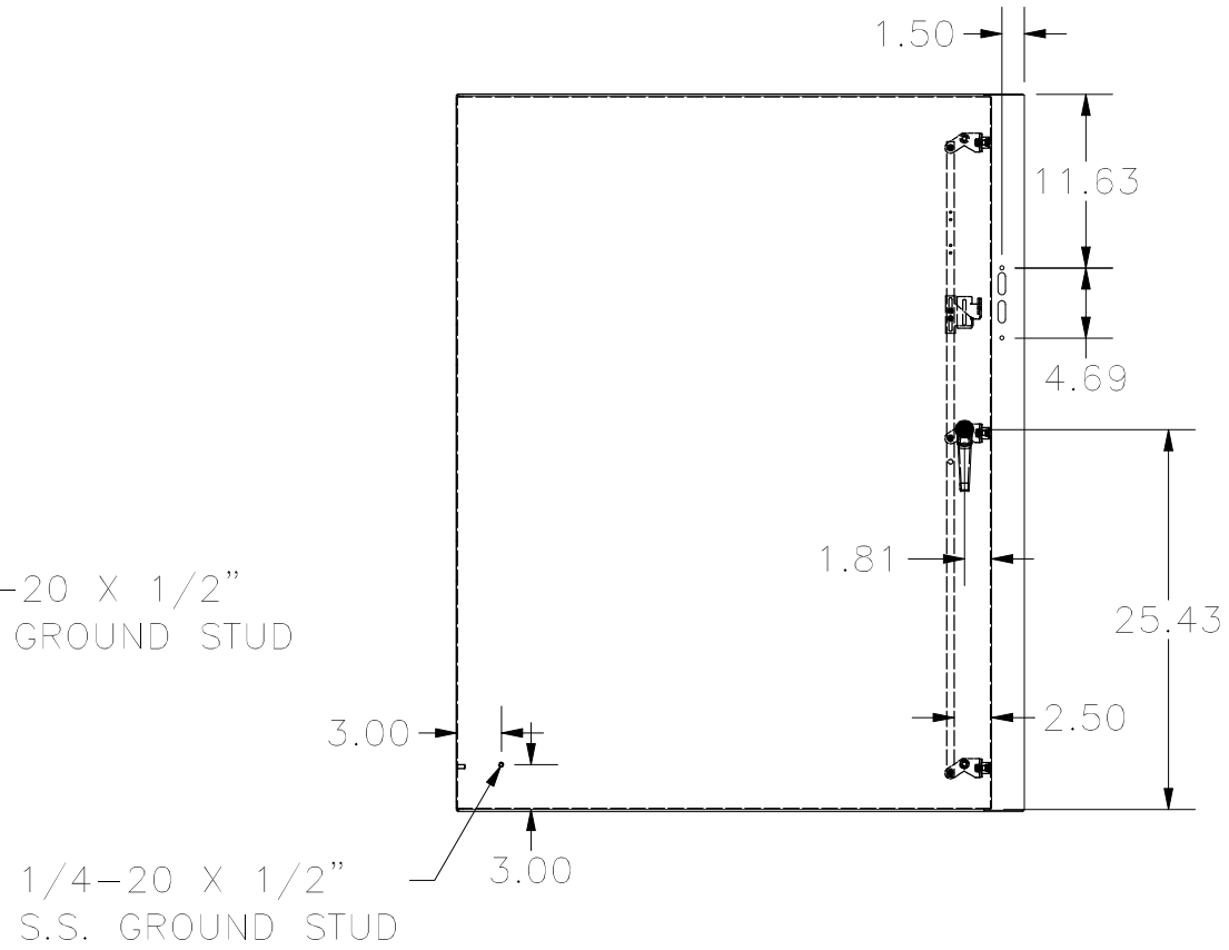
FRONT VIEW
