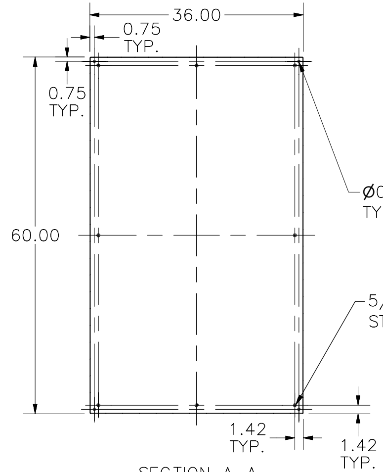
SECTION A-A (INSIDE BACK OF ENCLOSURE)
