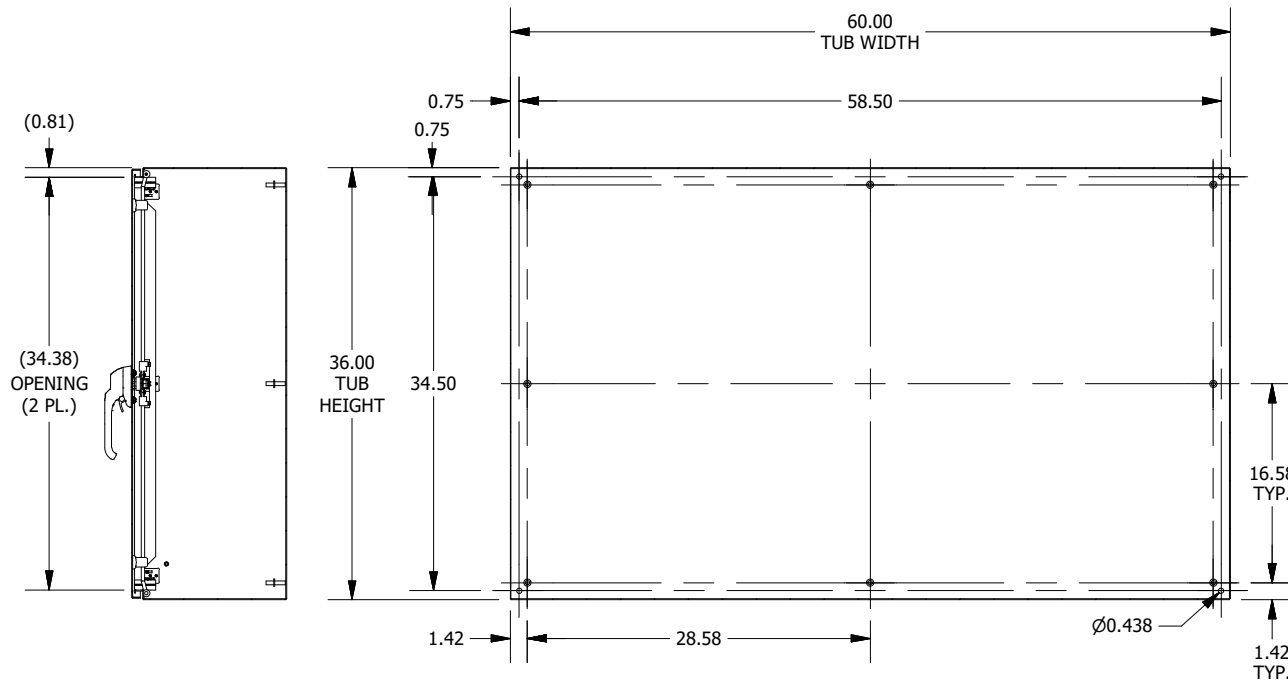
SECTION C-C (INSIDE LEFT OF ENCL.)
