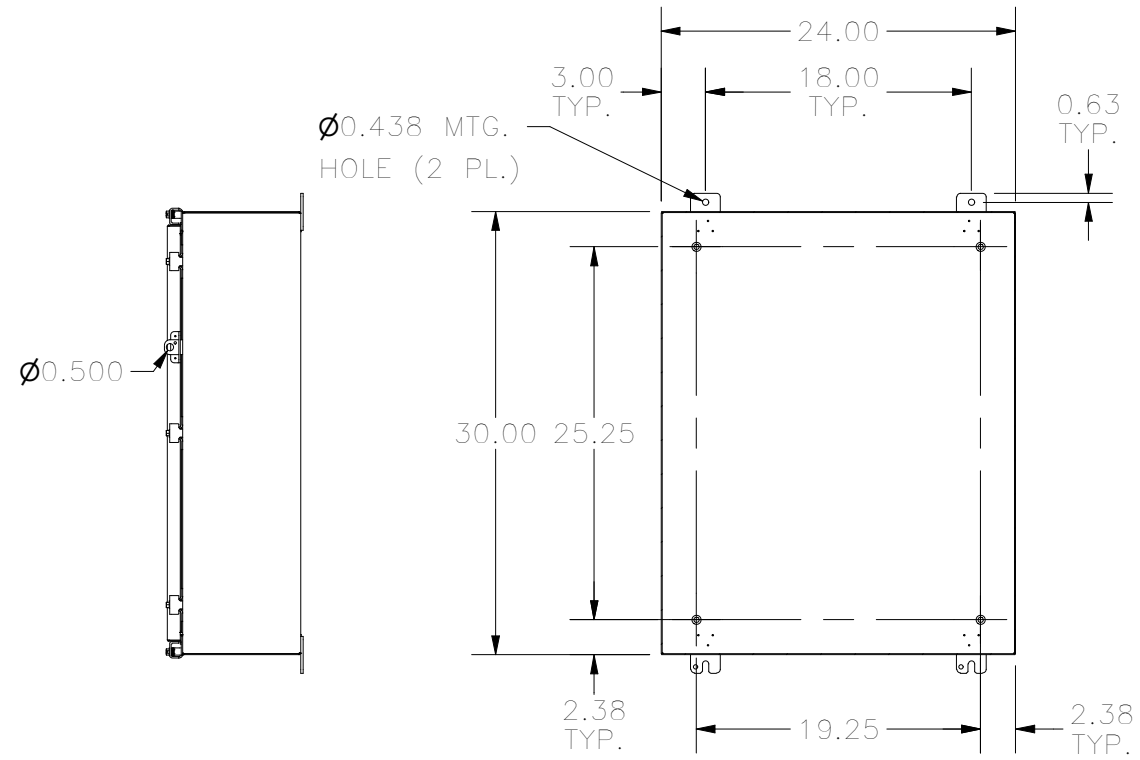
RIGHT VIEW
