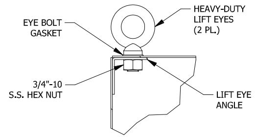
DETAIL AD (LIFT EYE ASSEMBLY VIEW)
