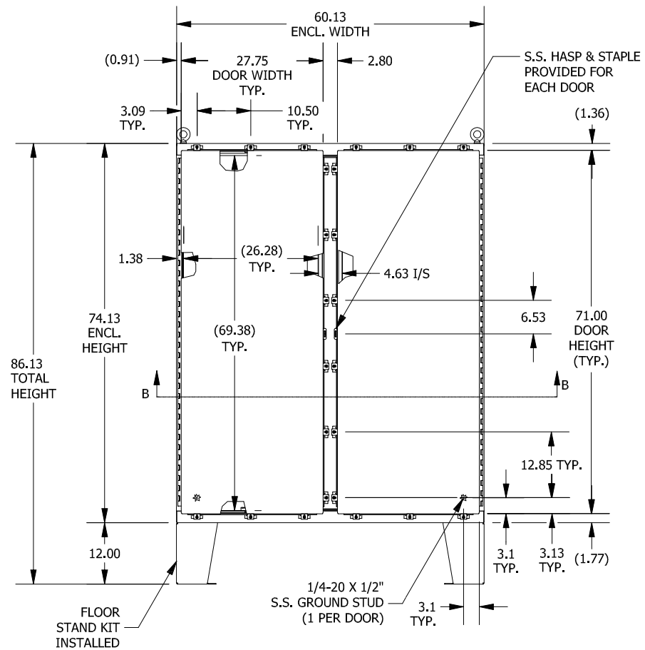
FRONT VIEW
