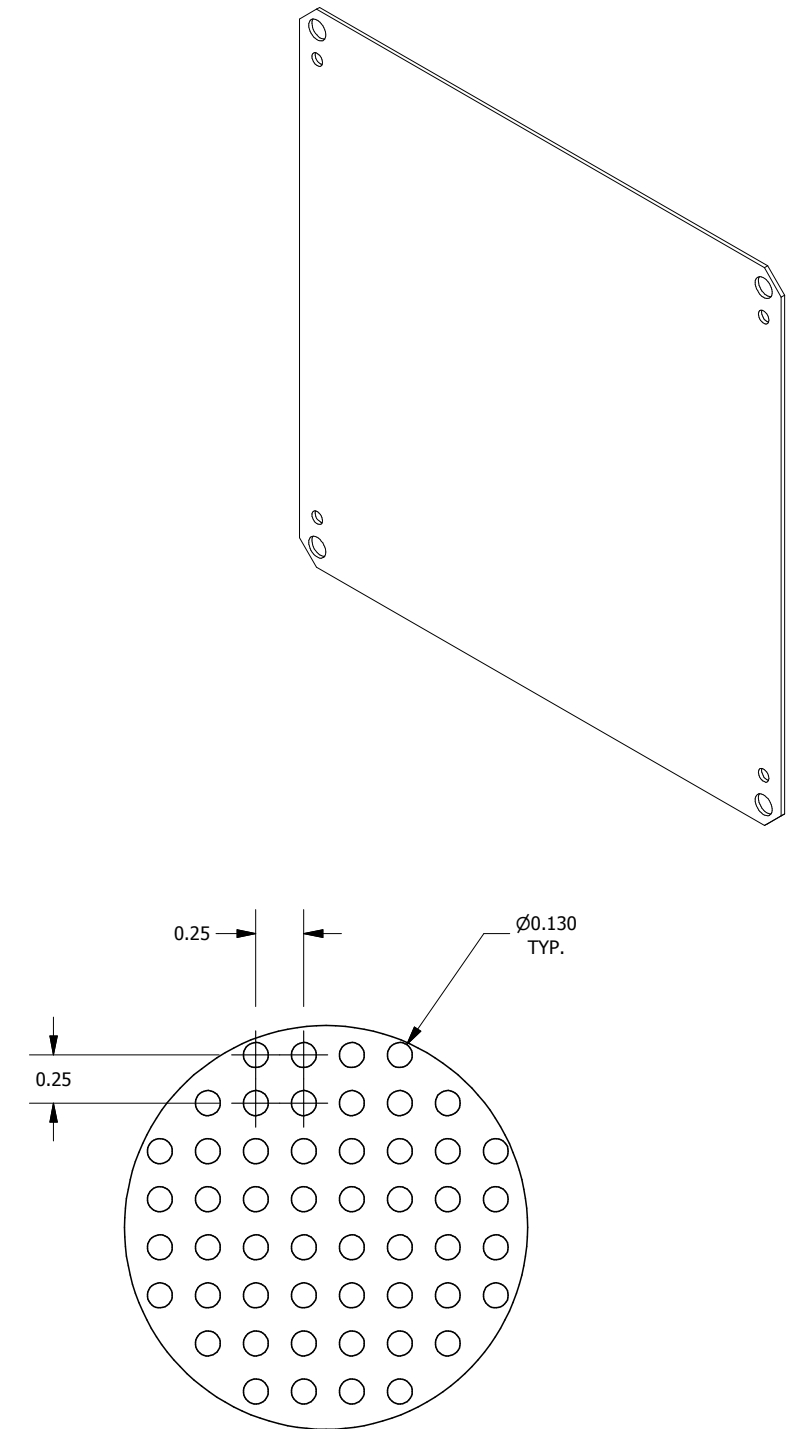
DETAIL-A (PERFORATED DETAIL)
