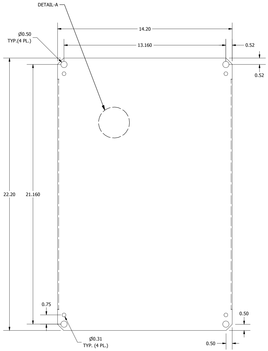
FRONT VIEW
