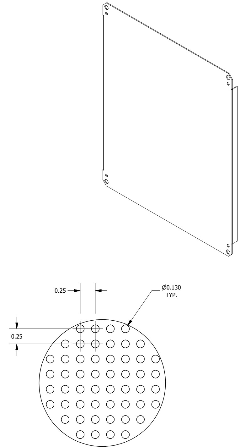
DETAIL-A (PERFORATED DETAIL)
