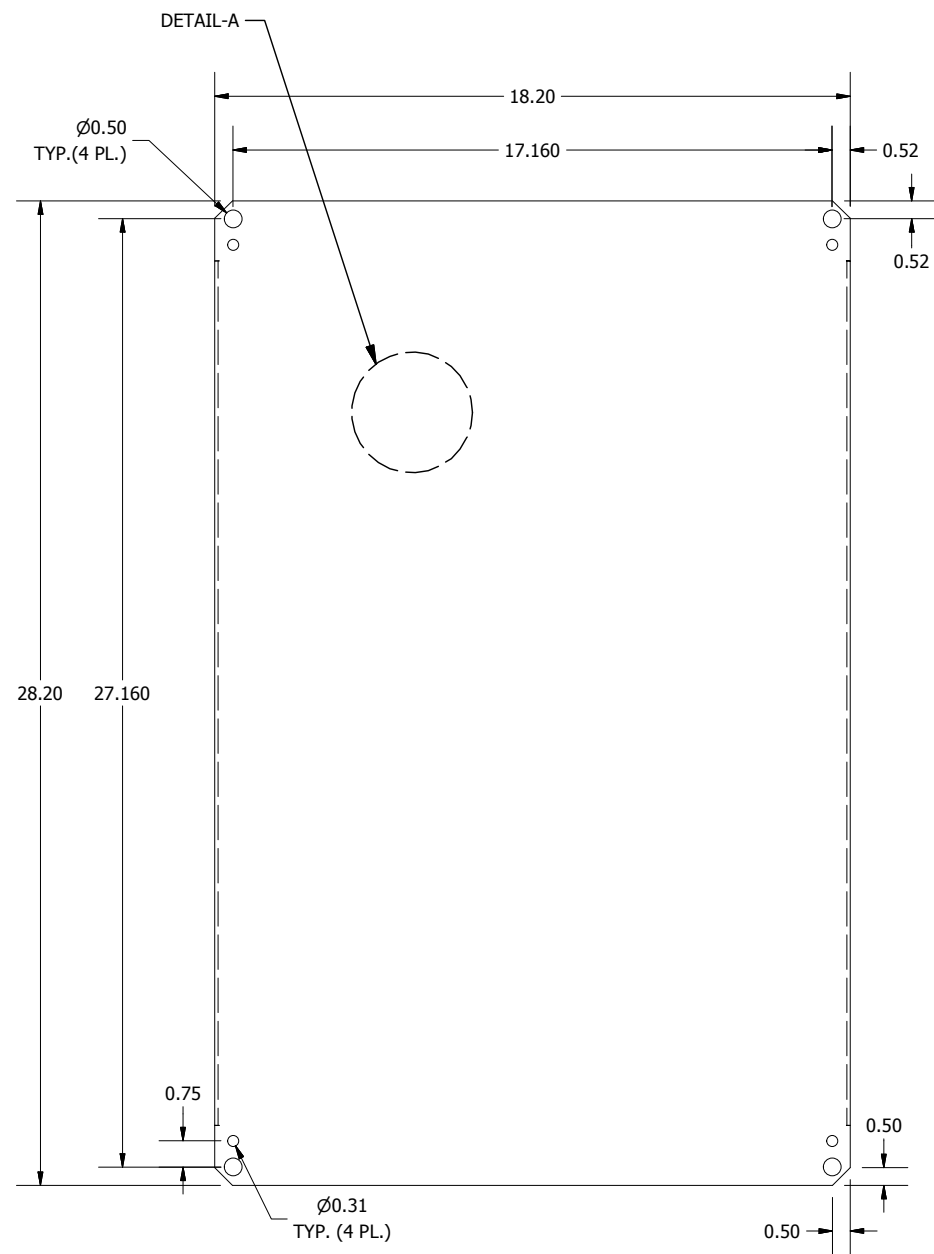
FRONT VIEW
