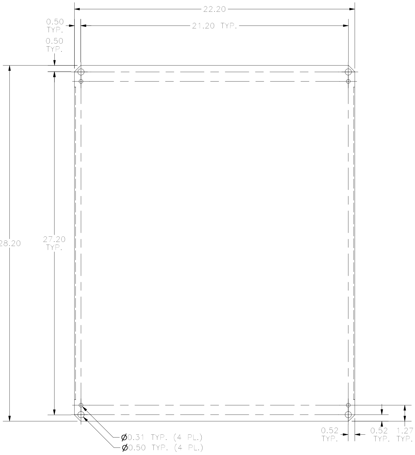
FRONT VIEW
