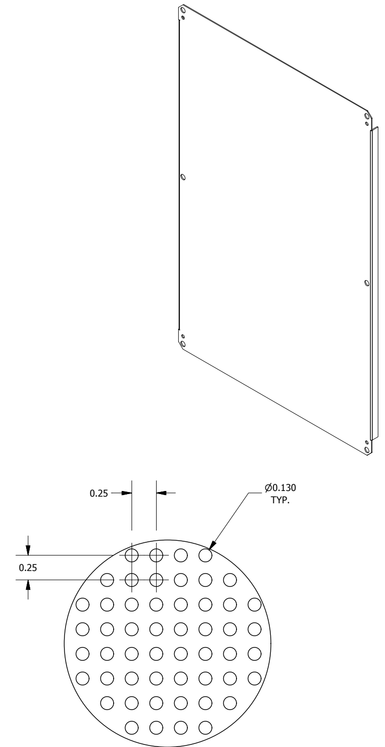
DETAIL-A (PERFORATED DETAIL)
