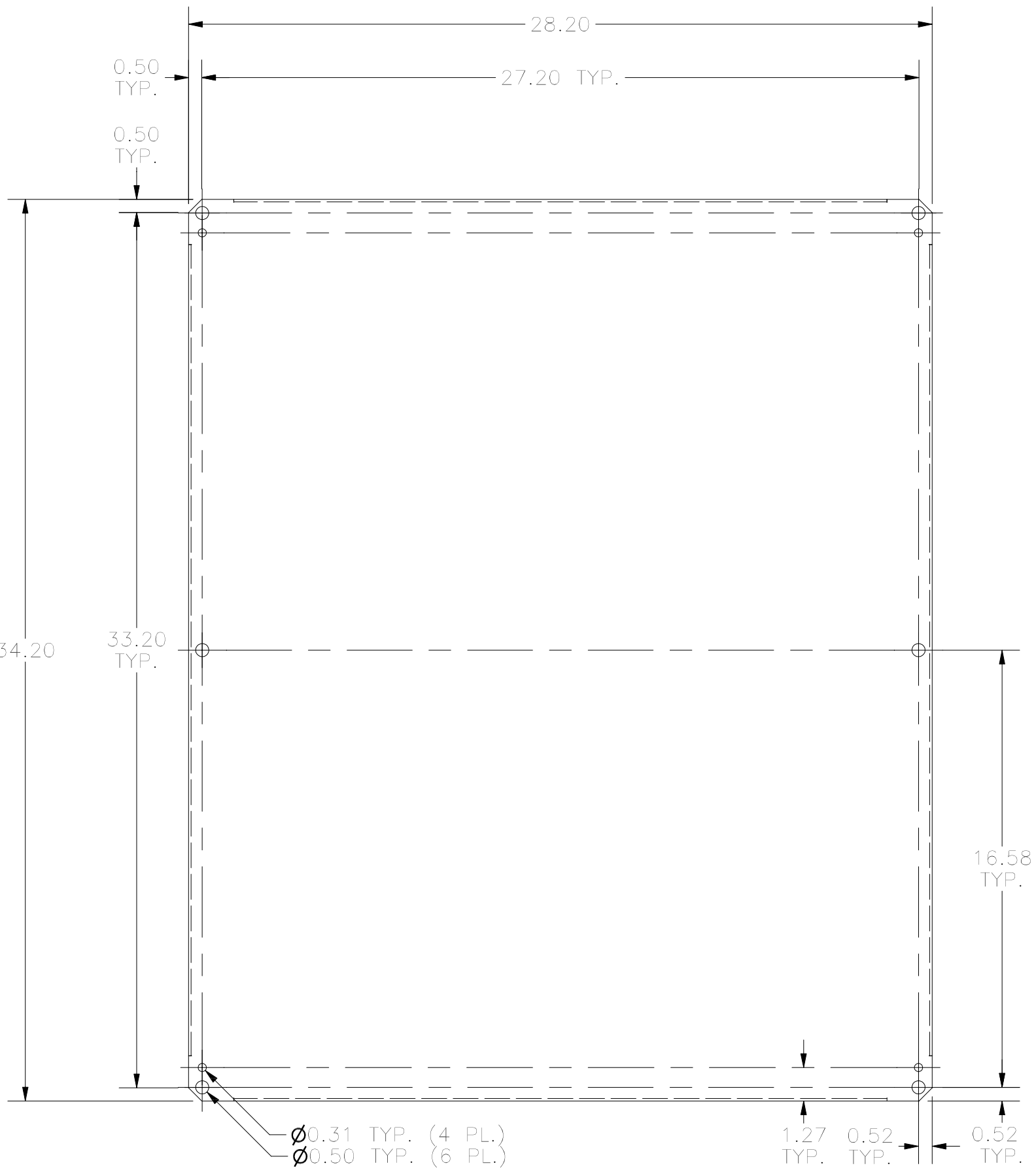
FRONT VIEW
