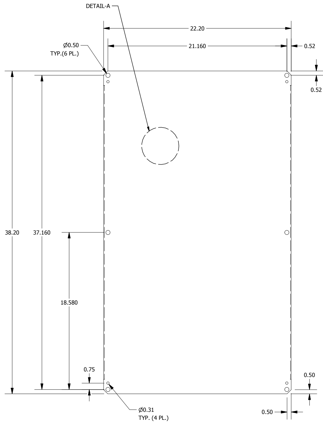
FRONT VIEW
