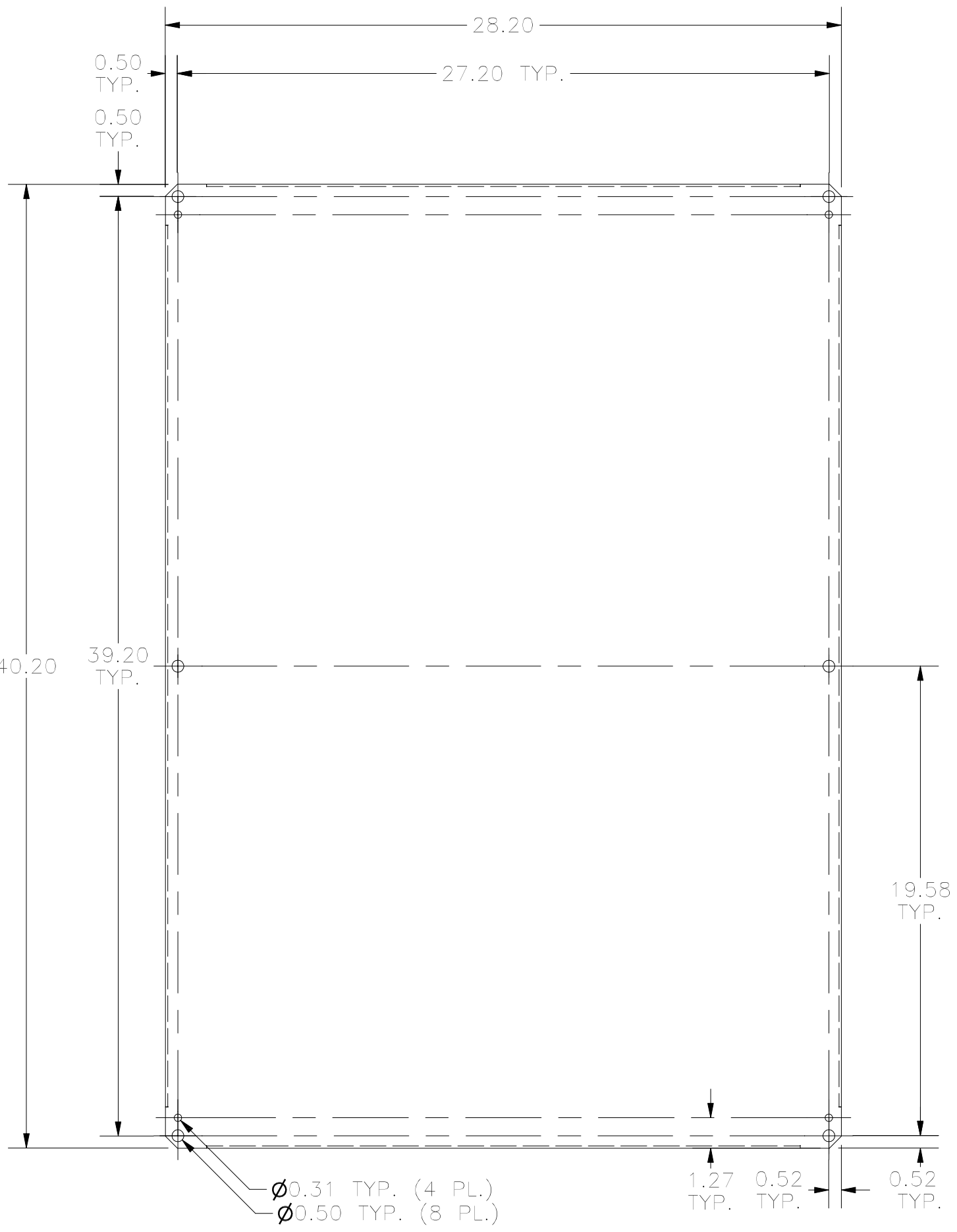
FRONT VIEW
