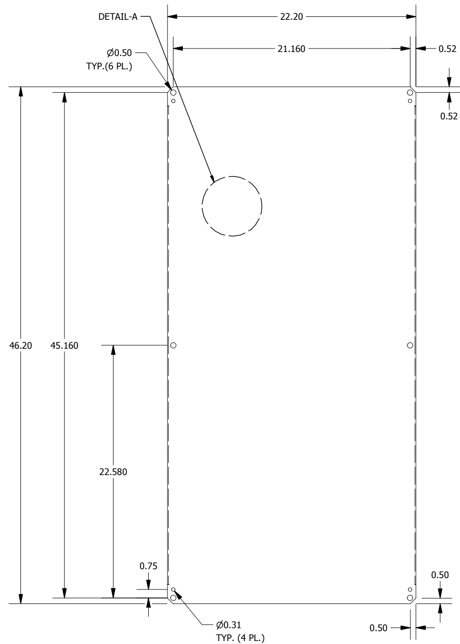
FRONT VIEW
