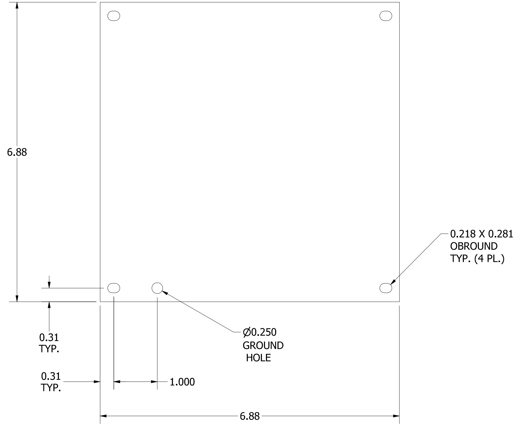
FRONT VIEW
