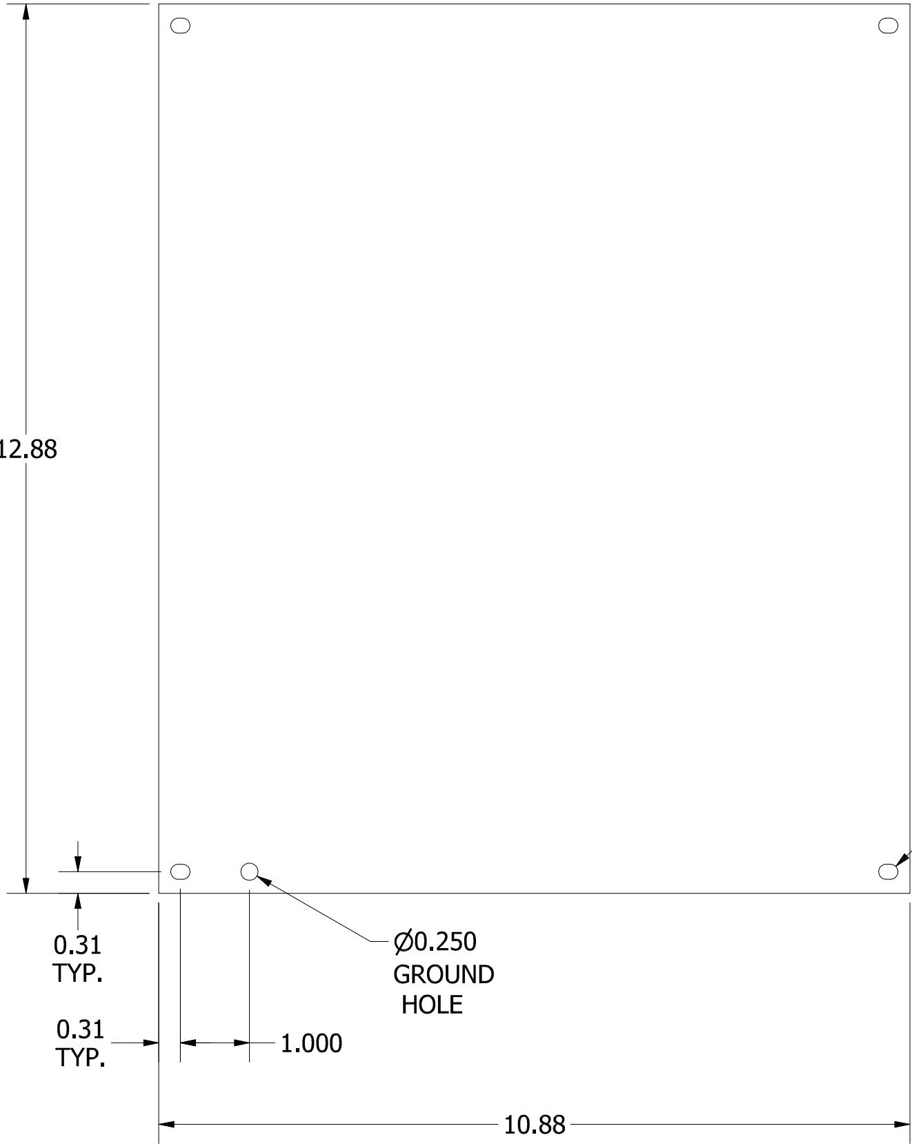
FRONT VIEW
