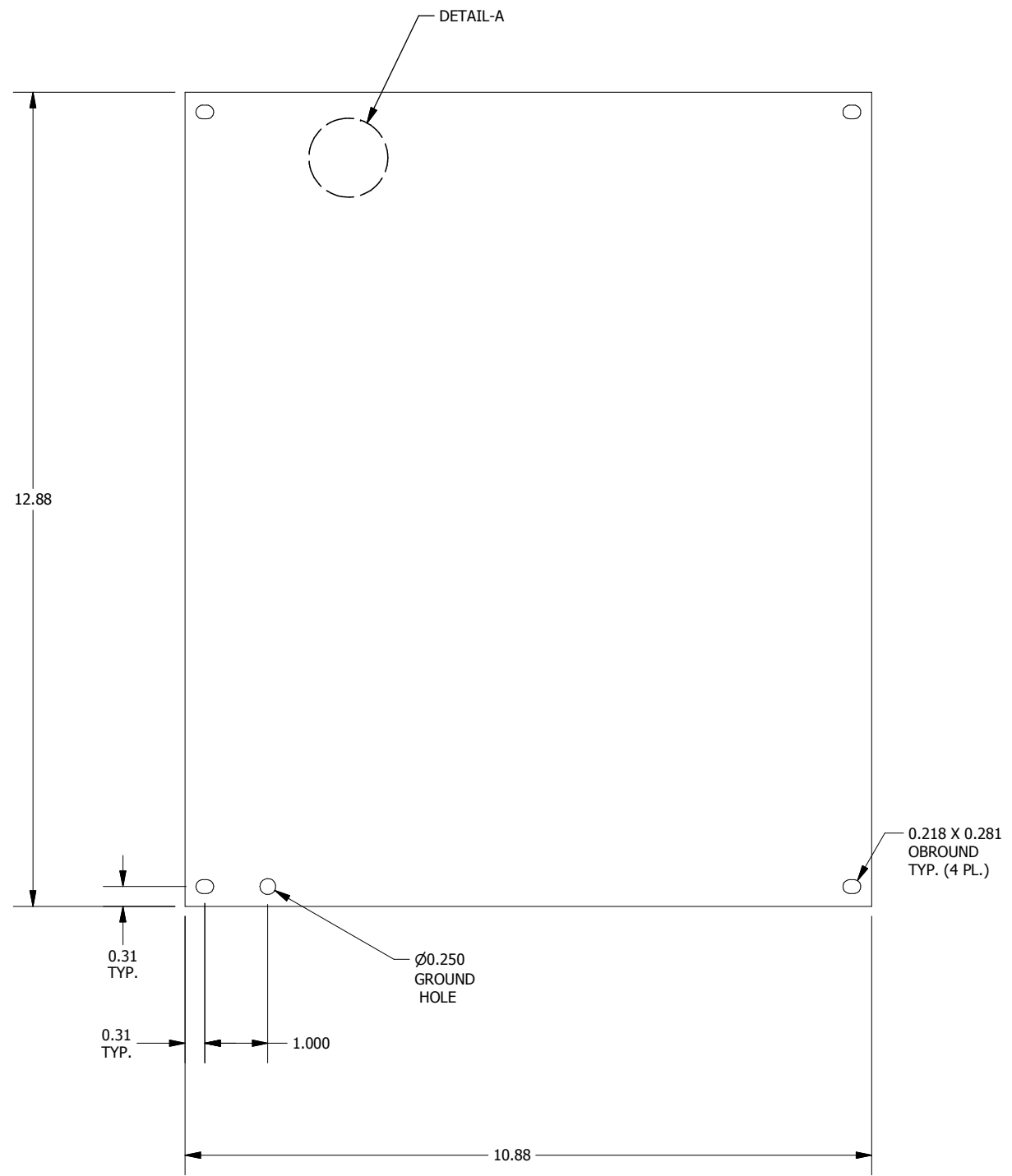
FRONT VIEW
