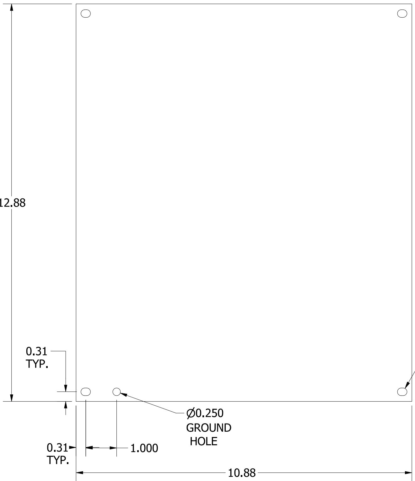
FRONT VIEW
