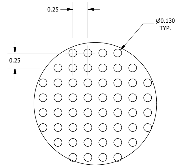
DETAIL-A (PERFORATED DETAIL)
