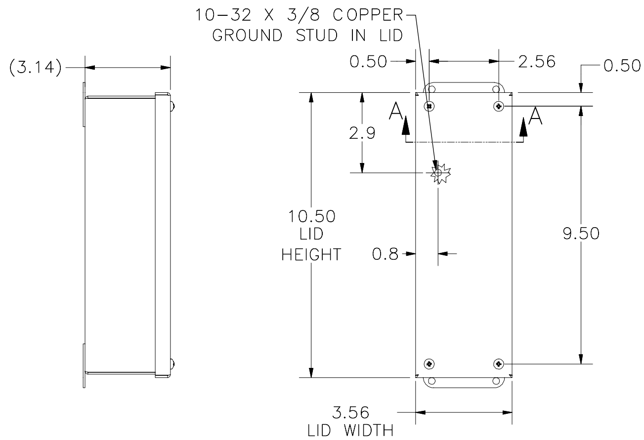
LEFT VIEW
