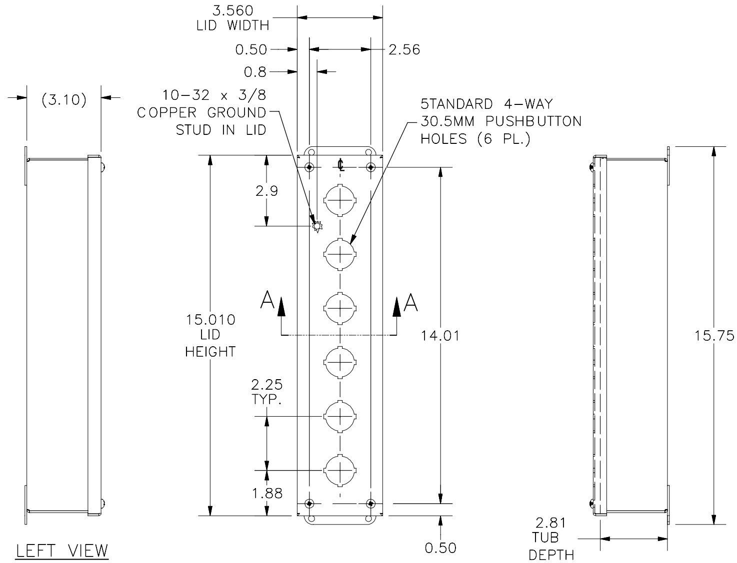
RIGHT VIEW
