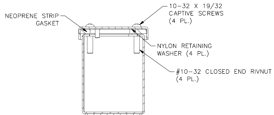
SECTION E-E (INSIDE TOP OF ENCLOSURE)
