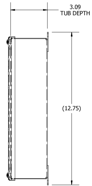
RIGHT VIEW
