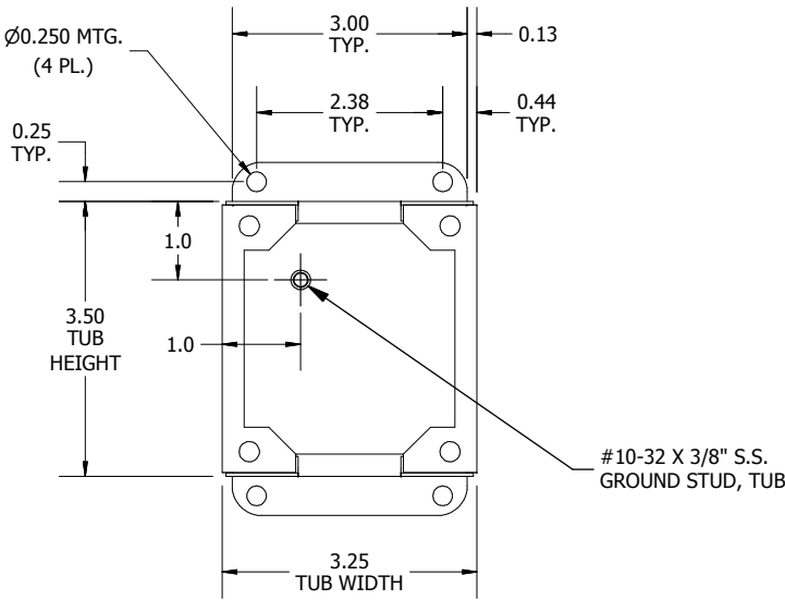
FRONT VIEW TUB
