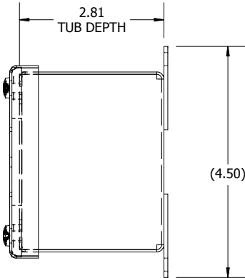
RIGHT VIEW
