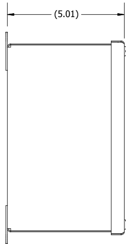
LEFT VIEW
