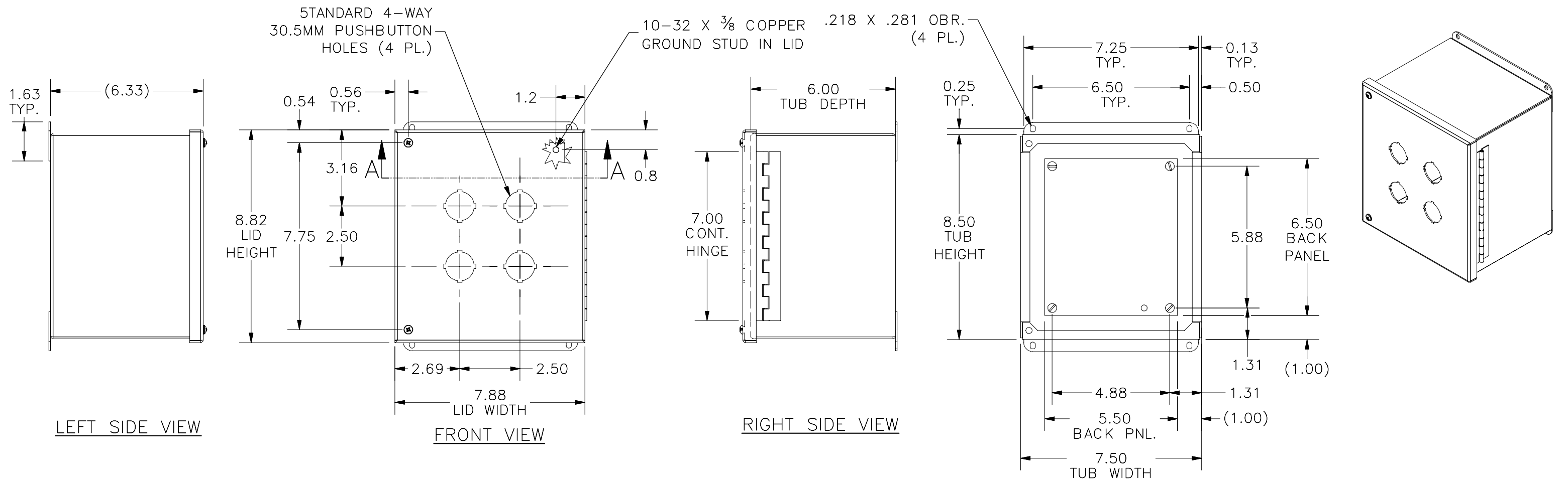
FRONT VIEW TUB (COVER REMOVED)
