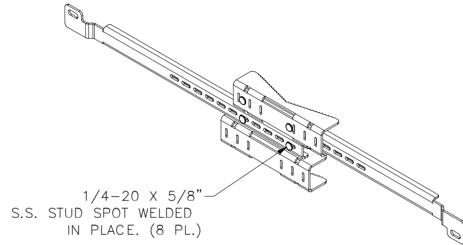
TOP BRACKET ISOMETRIC VIEW
