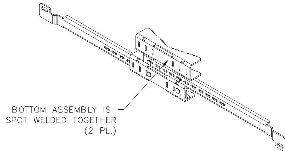
BOTTOM BRACKET ISOMETRIC VIEW
