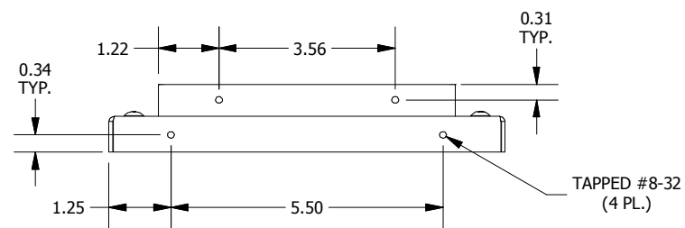
BOTTOM VIEW
