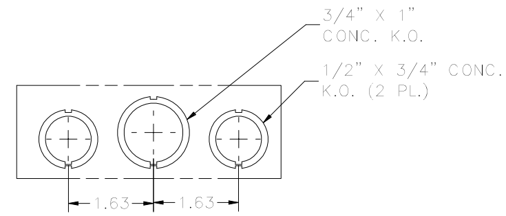
DETAIL C (KNOCKOUT DETAIL)
