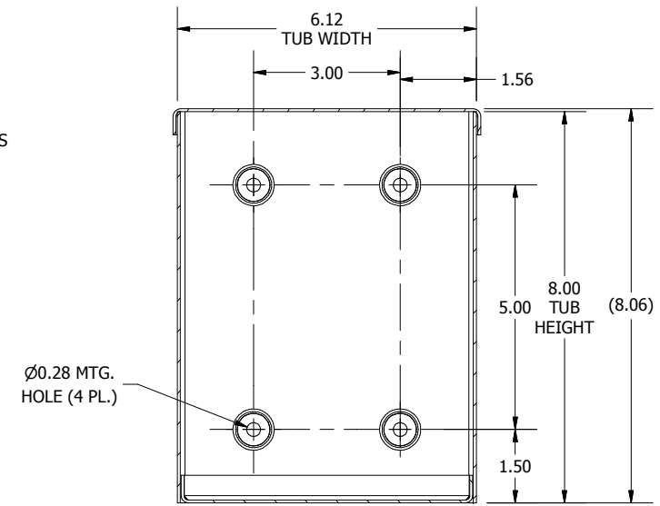
SECTION B-B (INSIDE BACK OF ENCL.)
