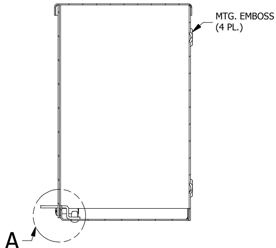
SECTION A-A (INSIDE LEFT OF ENCL.)
