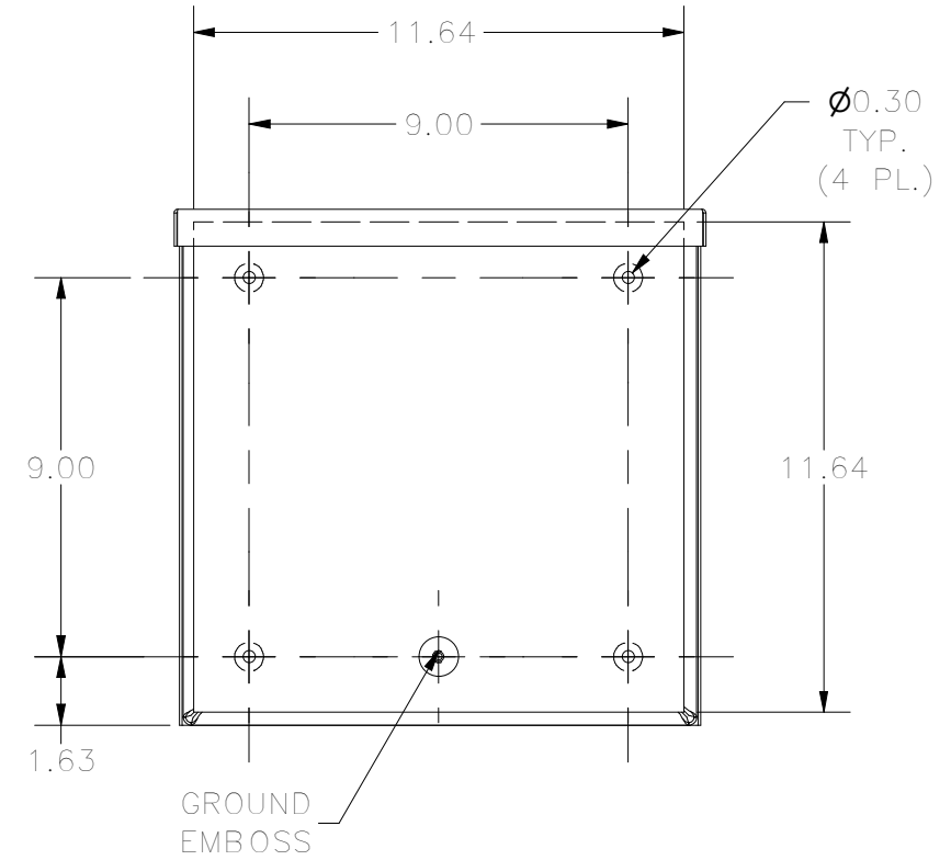
BACK VIEW
