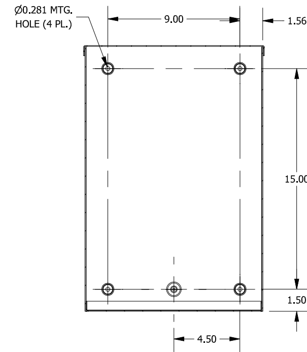
SECTION A-A (INSIDE BACK OF ENCL.)
