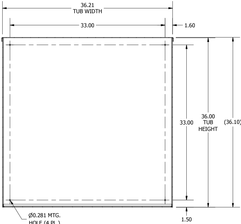
SECTION B-B (INSIDE BACK OF ENCL.)
