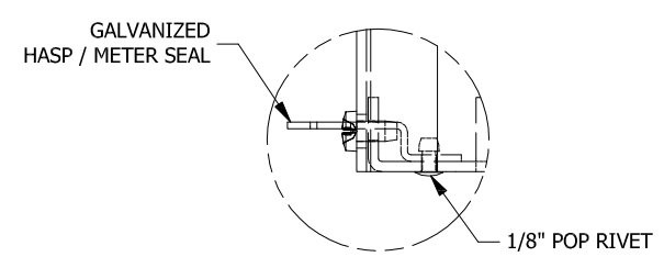
DETAIL A (METER SEAL DETAIL)
