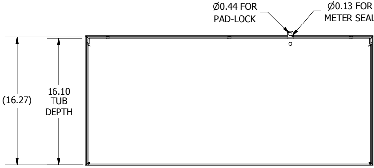
BOTTOM VIEW
