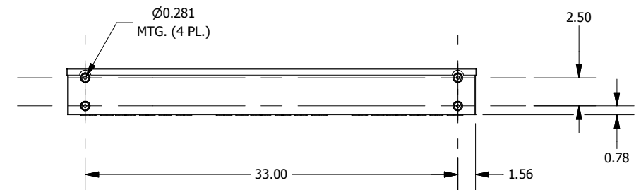
BACK VIEW
