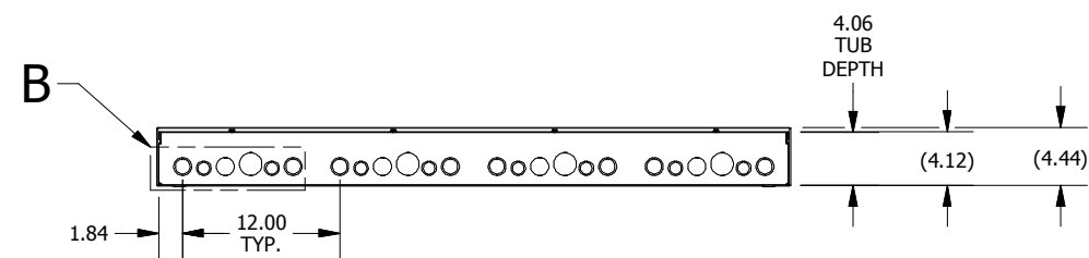
BOTTOM VIEW
