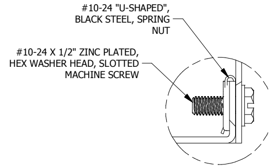
DETAIL A (4 PL.) (LID ATTACHMENT DETAIL)
